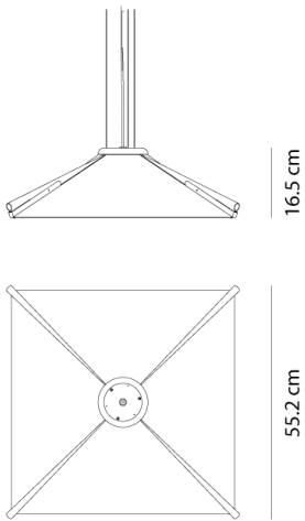
Product Dimensions
