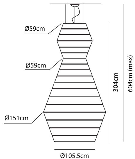
Product Dimensions
