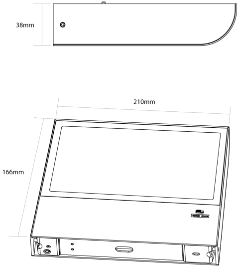
Product Dimensions
