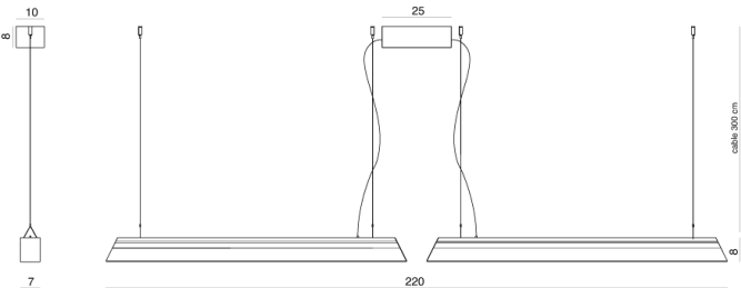
Product Dimensions
