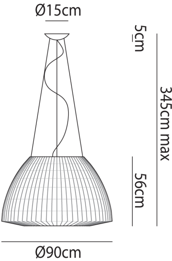
Product Dimensions
