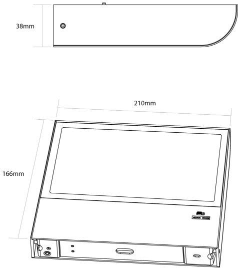
Product Dimensions
