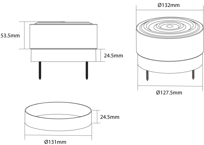
Product Dimensions
