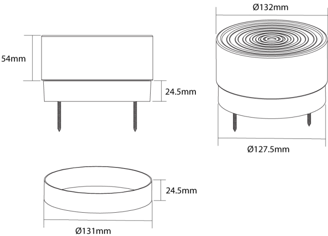
Product Dimensions
