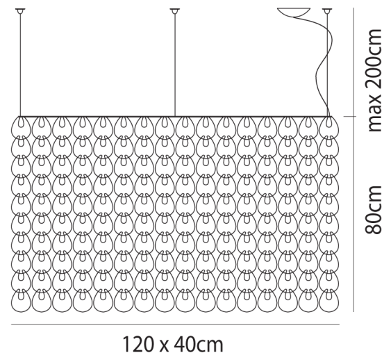
Product Dimensions
