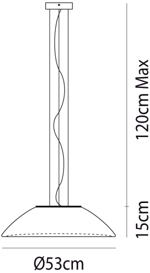
Product Dimensions
