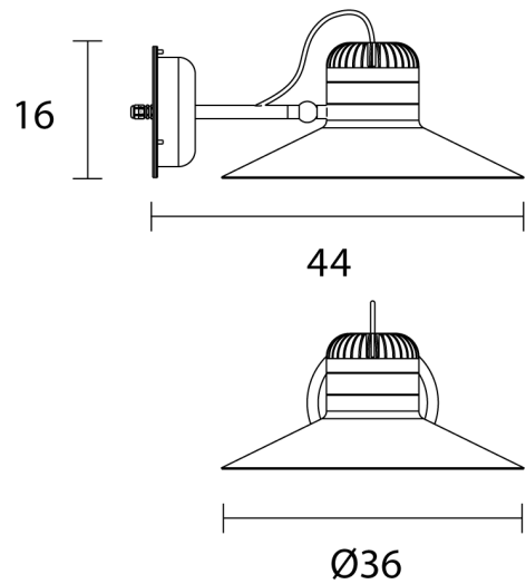
Product Dimensions
