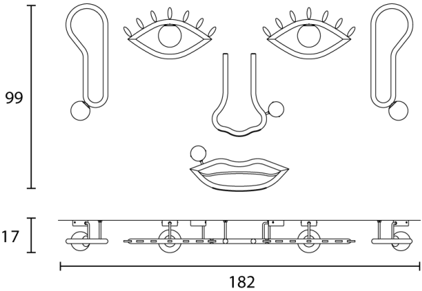
Product Dimensions
