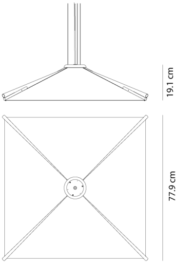
Product Dimensions
