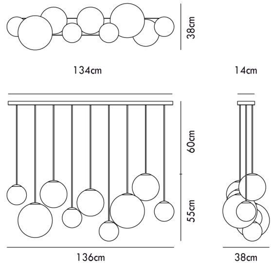
Product Dimensions
