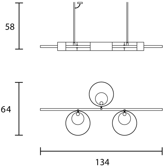
Product Dimensions
