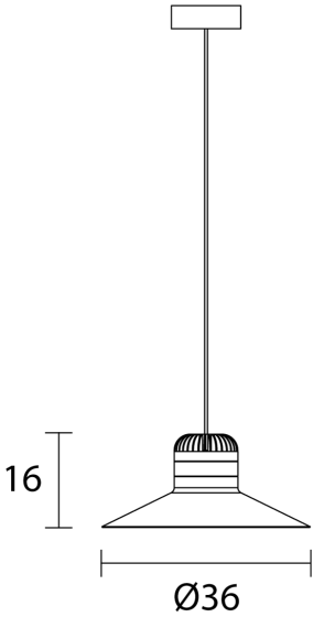
Product Dimensions
