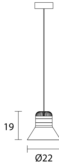
Product Dimensions
