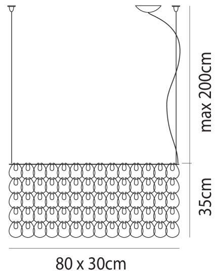
Product Dimensions
