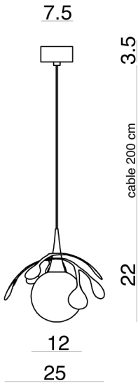
Product Dimensions
