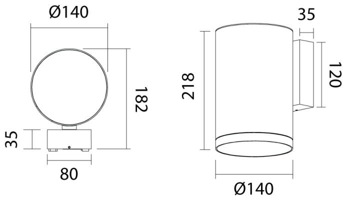
Product Dimensions
