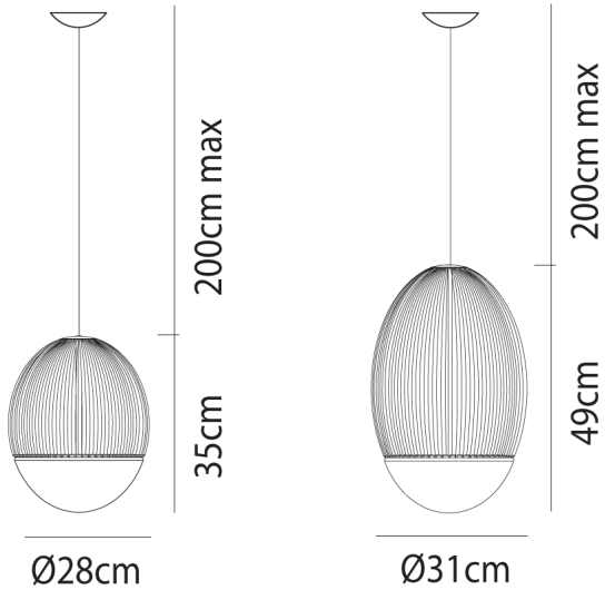
Product Dimensions
