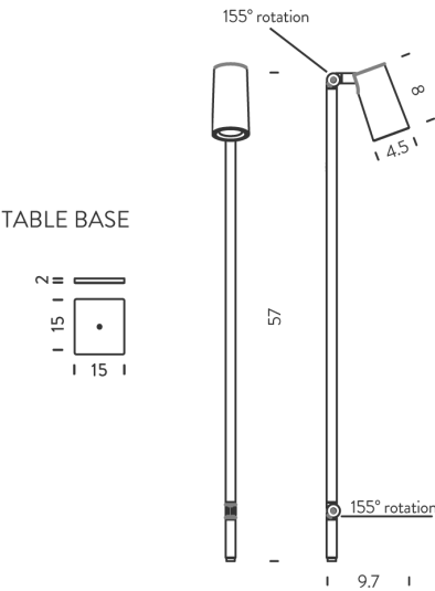
Product Dimensions
