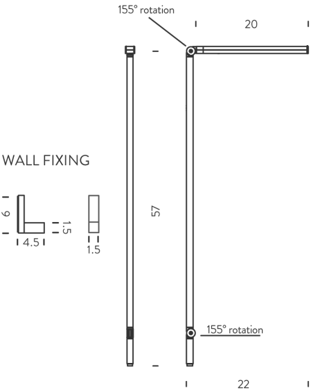
Product Dimensions
