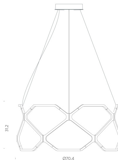
Product Dimensions
