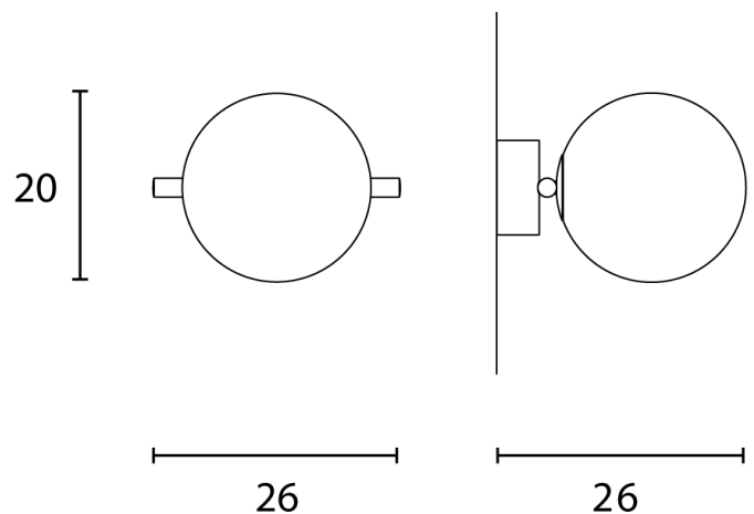
Product Dimensions
