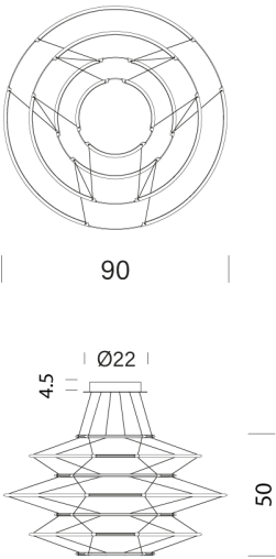
Product Dimensions
