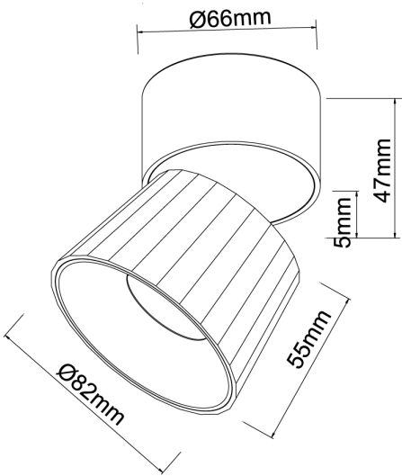
Product Dimensions
