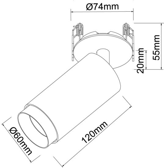
Product Dimensions
