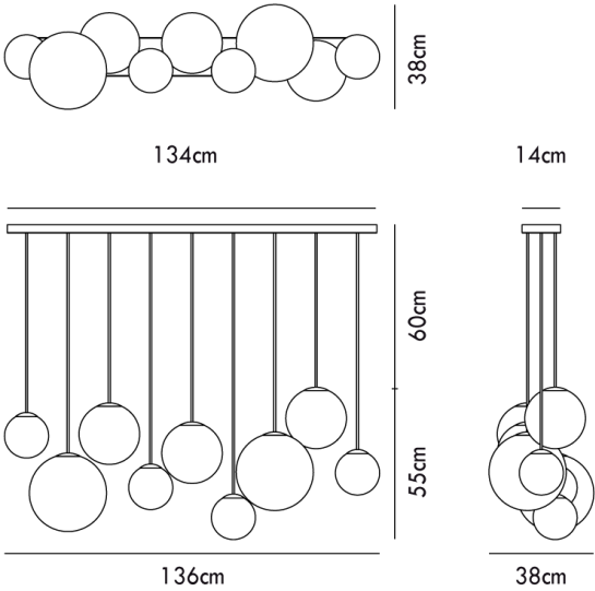
Product Dimensions
