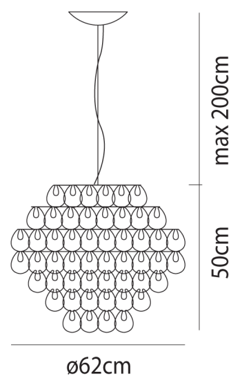
Product Dimensions
