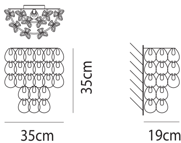
Product Dimensions
