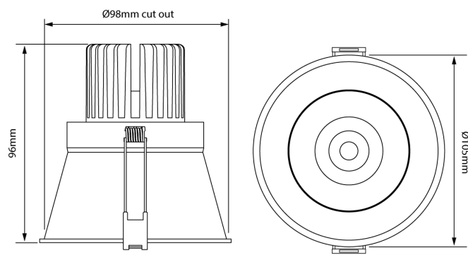
Product Dimensions
