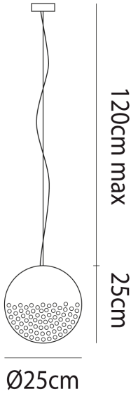
Product Dimensions
