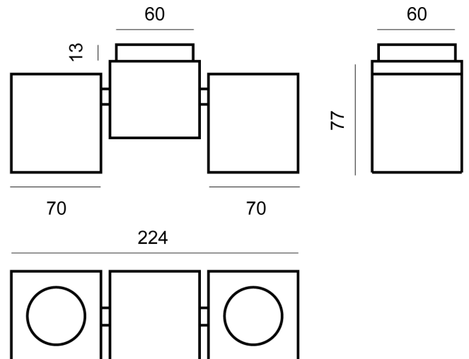
Product Dimensions
