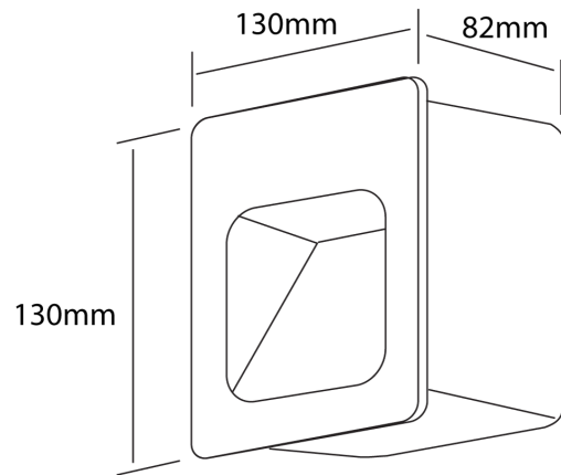
Product Dimensions
