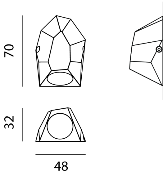
Product Dimensions
