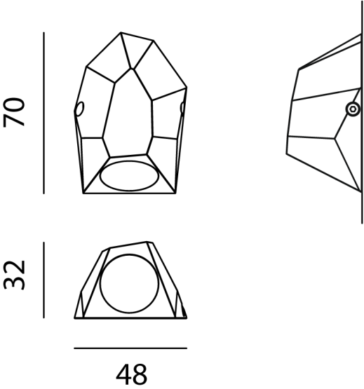
Product Dimensions
