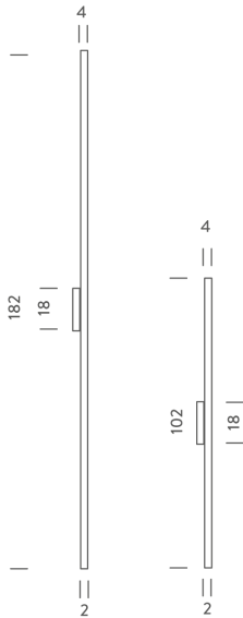
Product Dimensions
