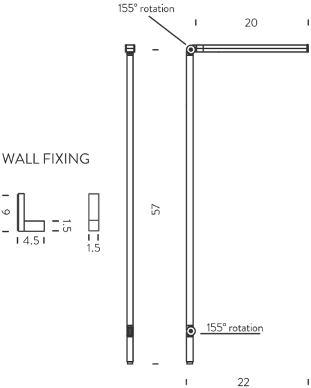
Product Dimensions
