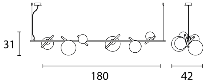
Product Dimensions
