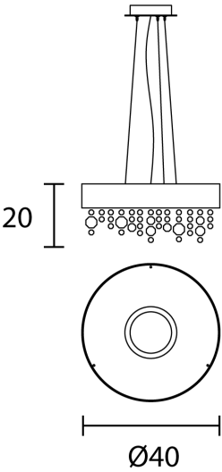
Product Dimensions
