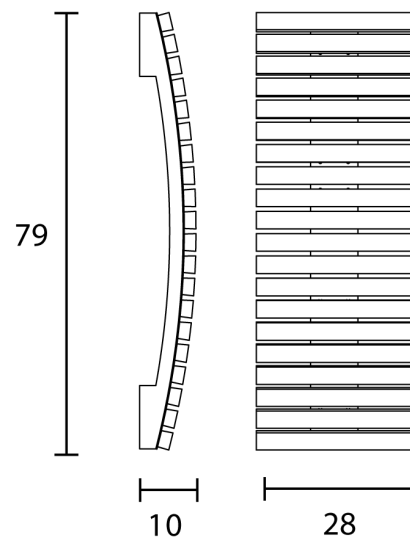
Product Dimensions
