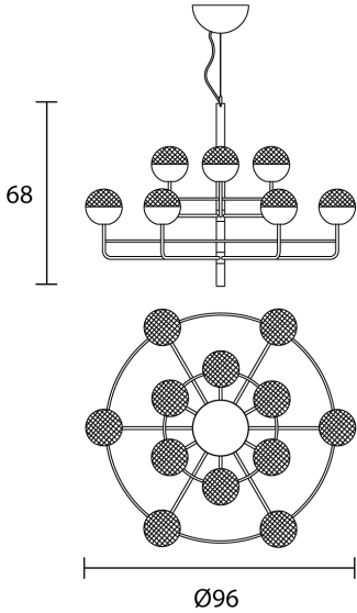
Product Dimensions
