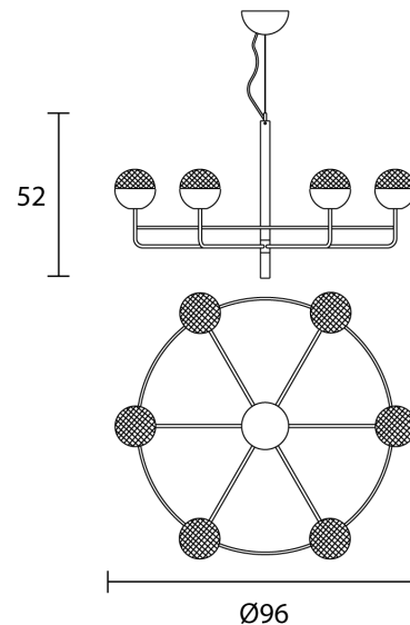
Product Dimensions
