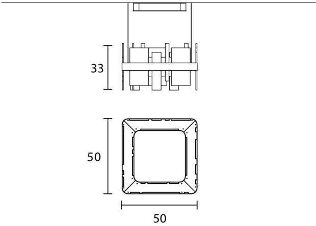
Product Dimensions
