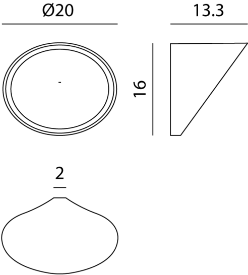
Product Dimensions
