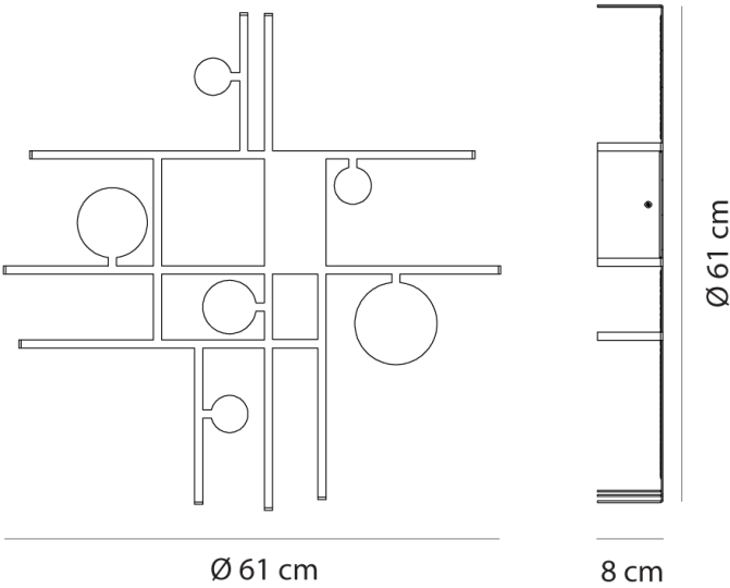
Product Dimensions
