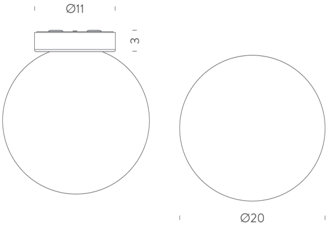
Product Dimensions
