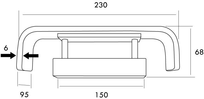
Product Dimensions
