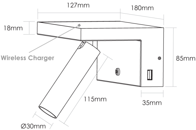
Product Dimensions
