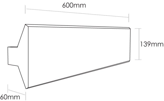
Product Dimensions
